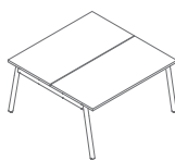
BOM44 1400 / 1410 / 740 61.6 kg
